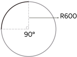
Curve Track Ø1200 mm / 90° R600
