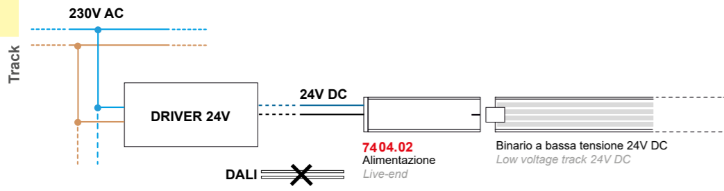
Schema cablaggio accensione ON/OFF Ignition ON/OFF Wiring Diagram
