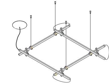
Example of installation with 4 art 0092 + 1 art 1671
