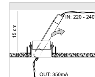
Installation without wall box 0206 - 0207
